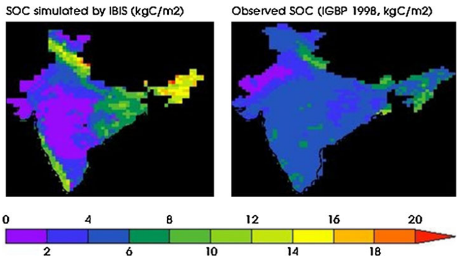
Fig. 8 Model simulated current SOC distribution compared with the observed SOC distribution
