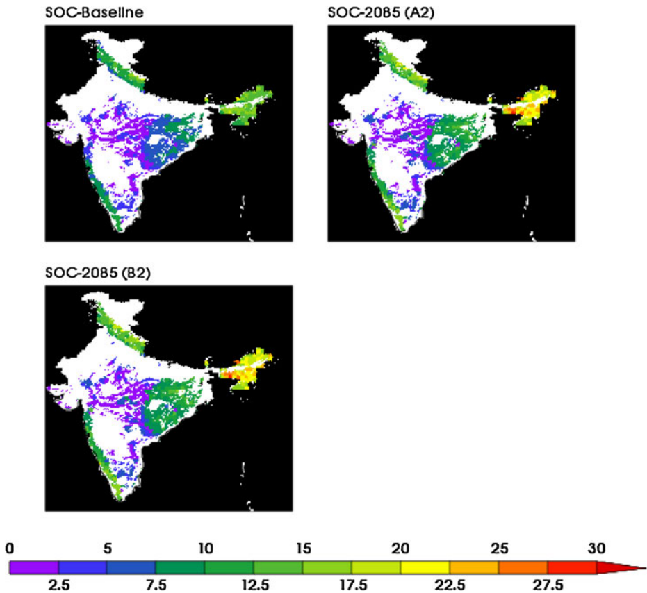
Fig. 16 Distribution of SOC ( \text{kgC/m}^2 ) simulated by IBIS for the baseline case and A2 and B2 scenarios
